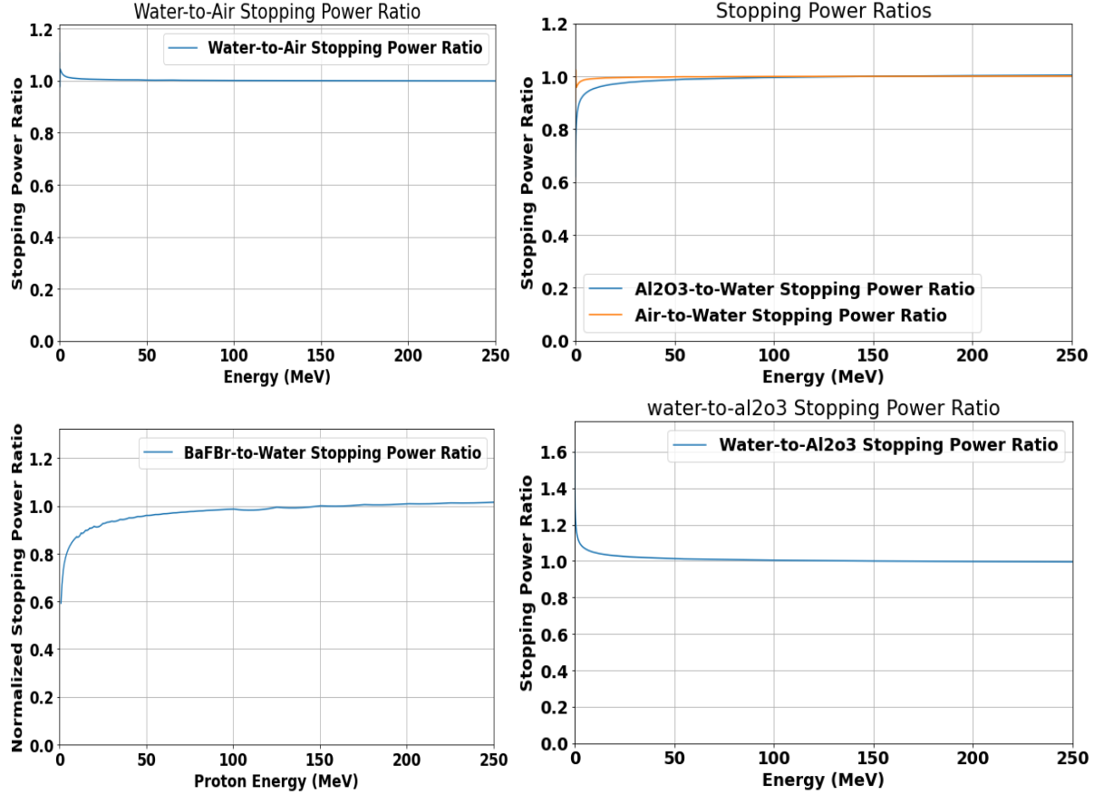
Figure 3: Stopping power ratios for materials like water, air, Al_2O_3 , and BaFBr over the 0-250 MeV proton energy range. The water-to-air ratio remains stable, while the Al_2O_3 -to-water and air-to-water ratios highlight their differing attenuation properties. The BaFBr-to-water ratio shows significant material-dependent differences, and the water-to- Al_2O_3 ratio is particularly relevant for proton therapy dosimetry calculations in medical physics. These ratios are crucial for normalizing dosimetry readings in proton therapy.
